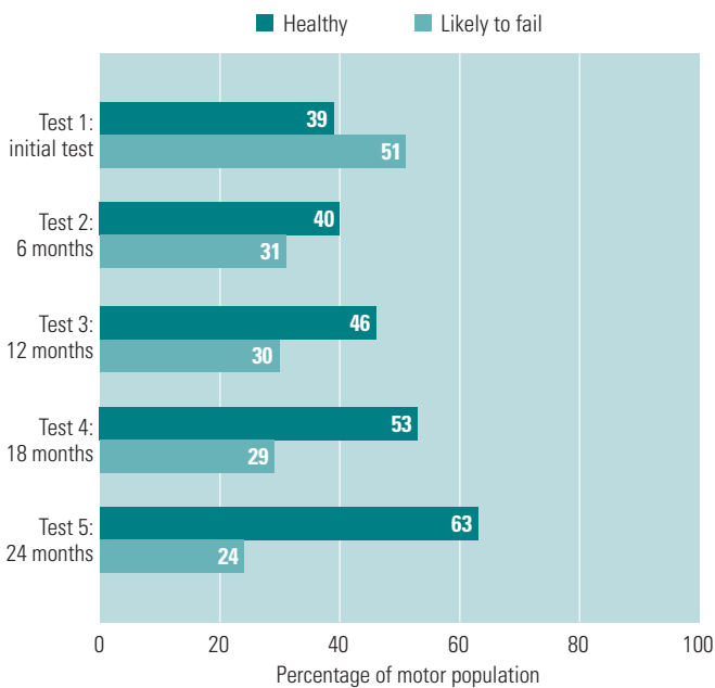
Figure 1: Results from ongoing MCA testing Consistent motor circuit analysis (MCA) testing and follow-up can dramatically improve the health of motor systems. Results are from repeated testing of approximately 1,000 motors.
