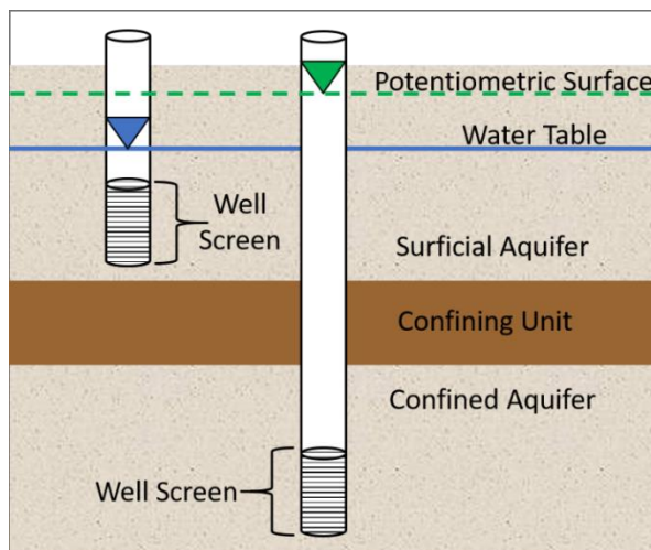
Figure 17. Illustration of a water table and potentiometric surface. Water levels in the wells are indicated by the blue (water table) and green (potentiometric surface) triangles.
