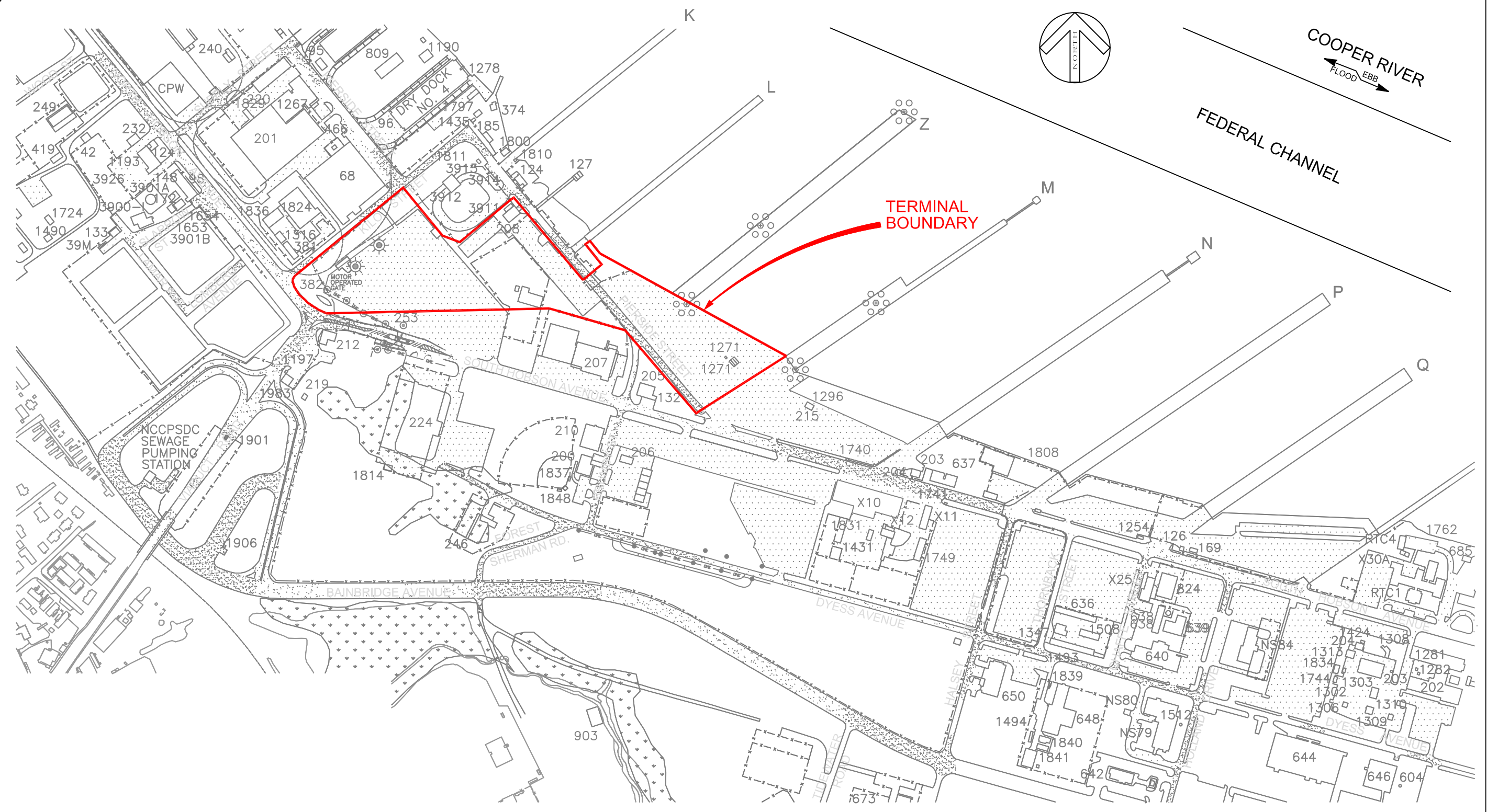
PLAN VIEW TERMINAL LAYOUT
