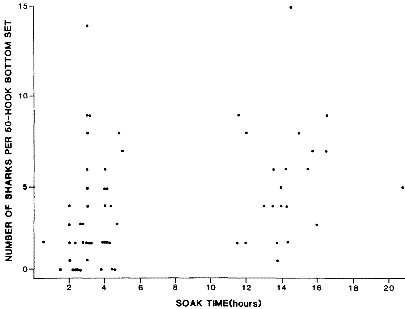
Fig. 2. CPUE (sharks/set) as a function of bottom longline soak time.
